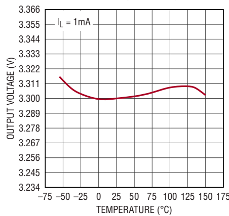
LT3066-3.3 Output Voltage
