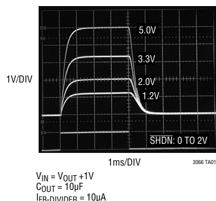
Output Discharge vs V_{OUT} C_{REF/BYP} = 1nF
