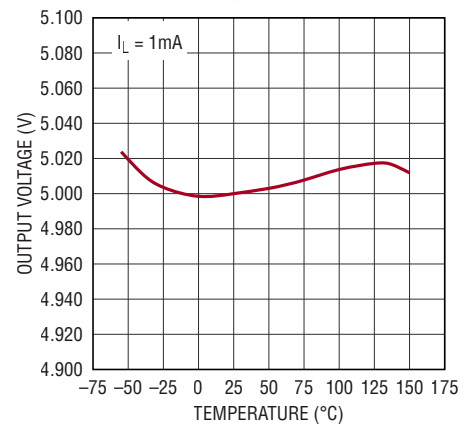
LT3066-5 Output Voltage
